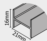
Panel connector
