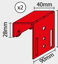
LA001002 Upper travel hardware
