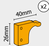
LA002230 End catch
