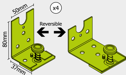
LA003302 Lower travel hardware
