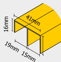
LA00A0F3 Aluminium double lower guide rail
