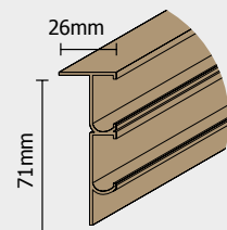
LA00K051 Aluminium double upper guide rail
