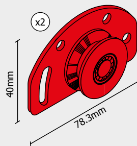
LA004411 Lower guide hardware with bearing Ø34mm
