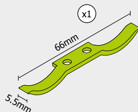
LA004413 Guide Latch
