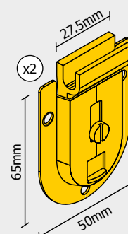
LA004412 Upper guide hardware with metal casing
